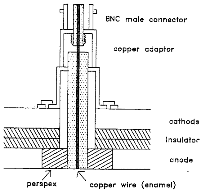
Fig. 3.11 The design of C_1 .
