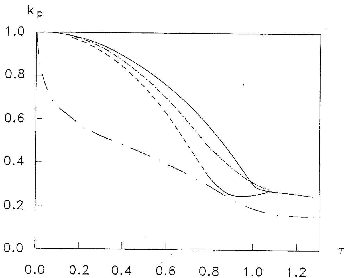
Fig. 4.2 Normalised radial trajectories of the magnetic piston, k_p vs normalised time, \tau of a 0.8 mbar hydrogen pinch driven by the first bank alone.
