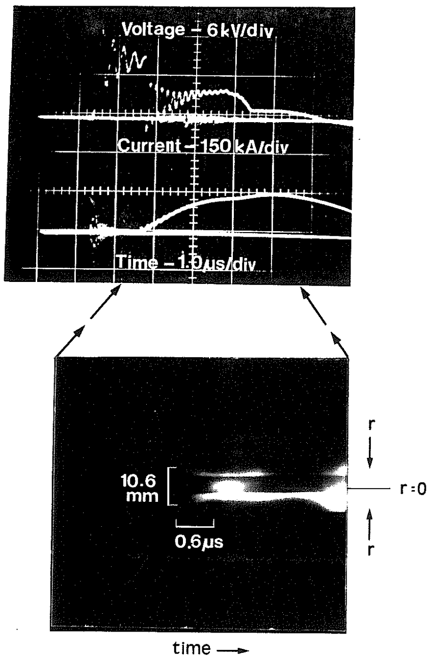
Fig. 4.1 The electrical signals and the corresponding streak photograph showing the radial compression of a hydrogen pinch at 0.8 mbar driven by the first bank alone (without current-stepping).
