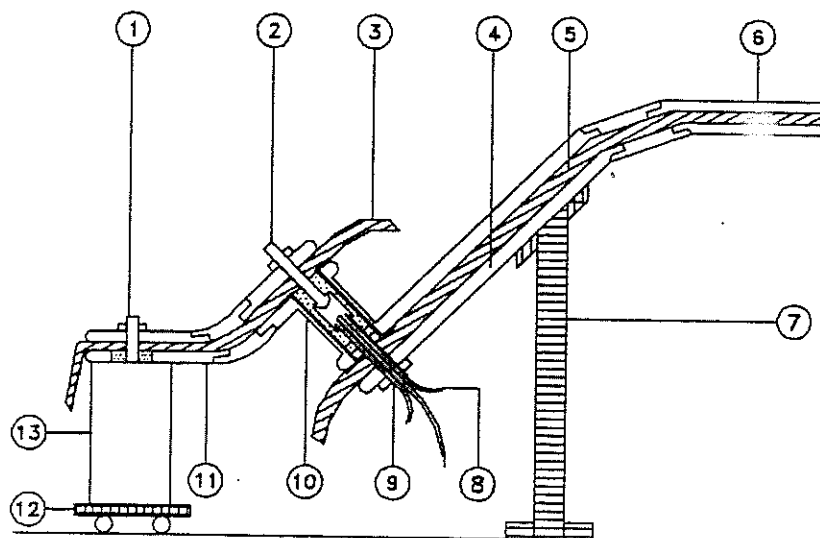
Fig. 3.5 Cross sectional view of one of the arms in Fig. 3.4 showing the connections between the capacitor, the pressurised spark gap and the anode flange. (reproduced from original diagram of KFA, IPP, 45 02 00-1 )
