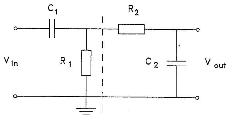
Fig. 3.10 The principle of the voltage probe.
