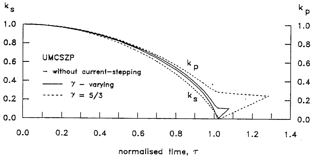
Fig. 6.13 Piston and shock trajectories with \gamma - varying and \gamma = 5/3 of UMCSZP.
